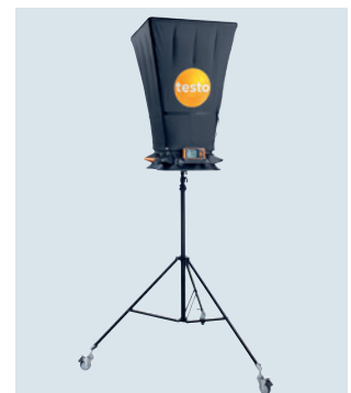
Stable, wheeled tripod with central fitting for secure working at high ceiling outlets.
