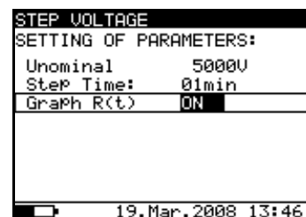
Fig. 25. Set-up menu in Step Voltage measurement
