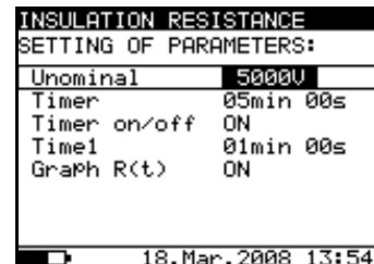
Fig. 12. Set-up menu in Insulation Resistance measurement
