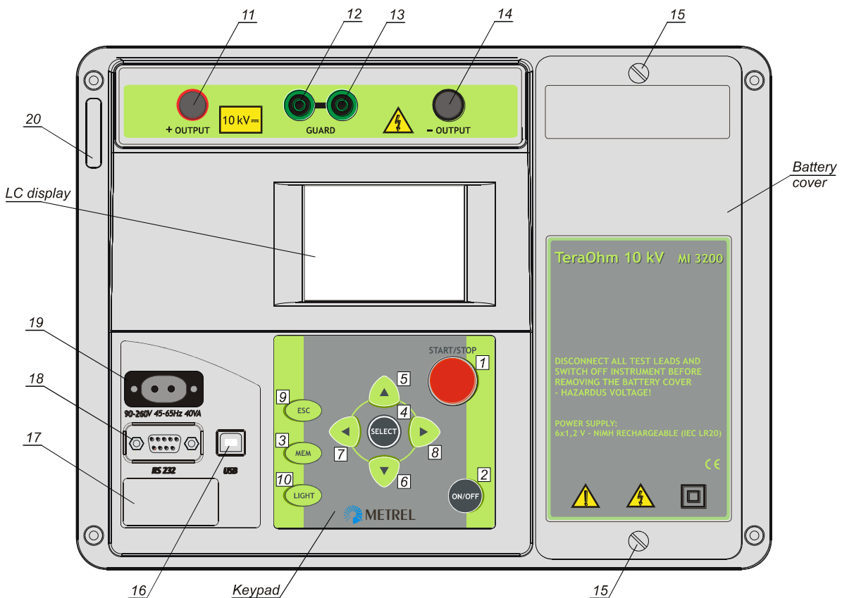
Fig. 1. Front panel
