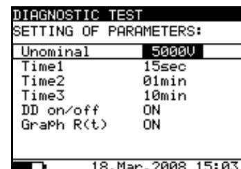
Fig. 17. Set-up menu in Diagnostic Test
