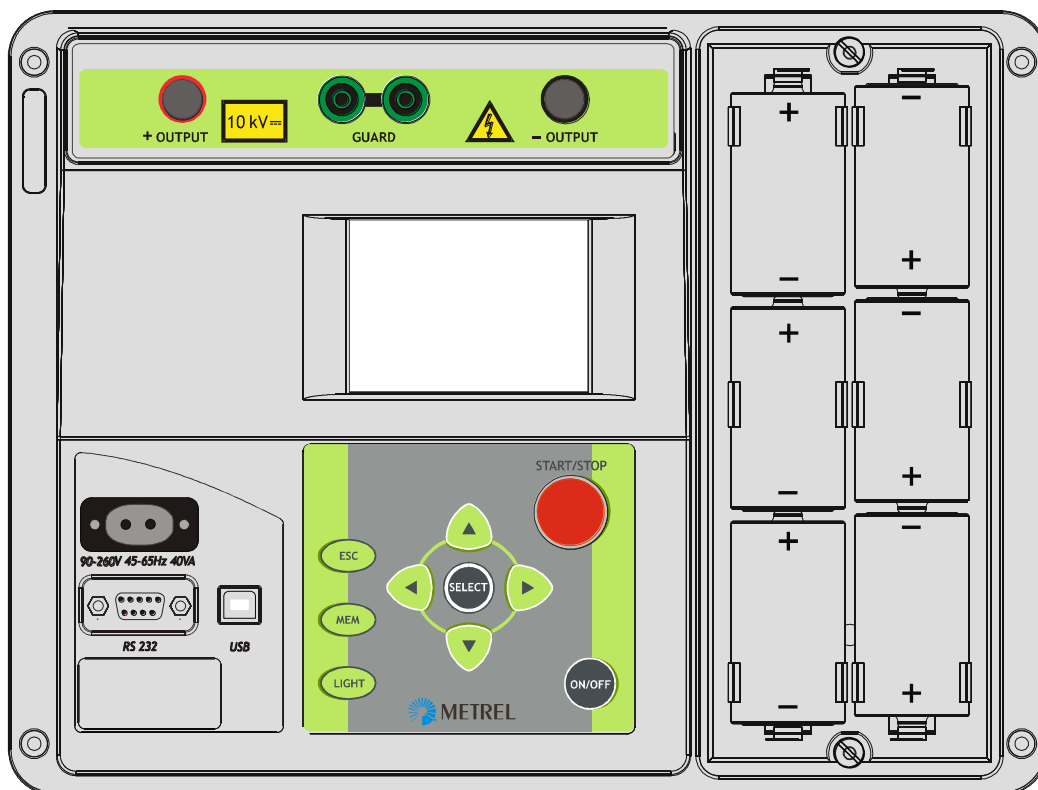
Fig. 31. Correct polarity of inserted batteries
