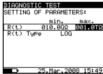
Fig. 20. Set-up menu of the Graph R(t)
