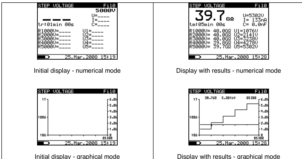
Fig. 22. Step Voltage function display states - Graph R(t) enabled
