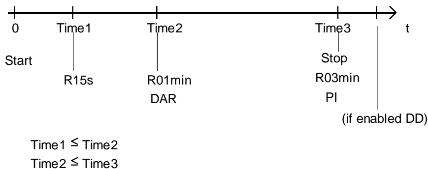
Fig. 18. Timer relations
