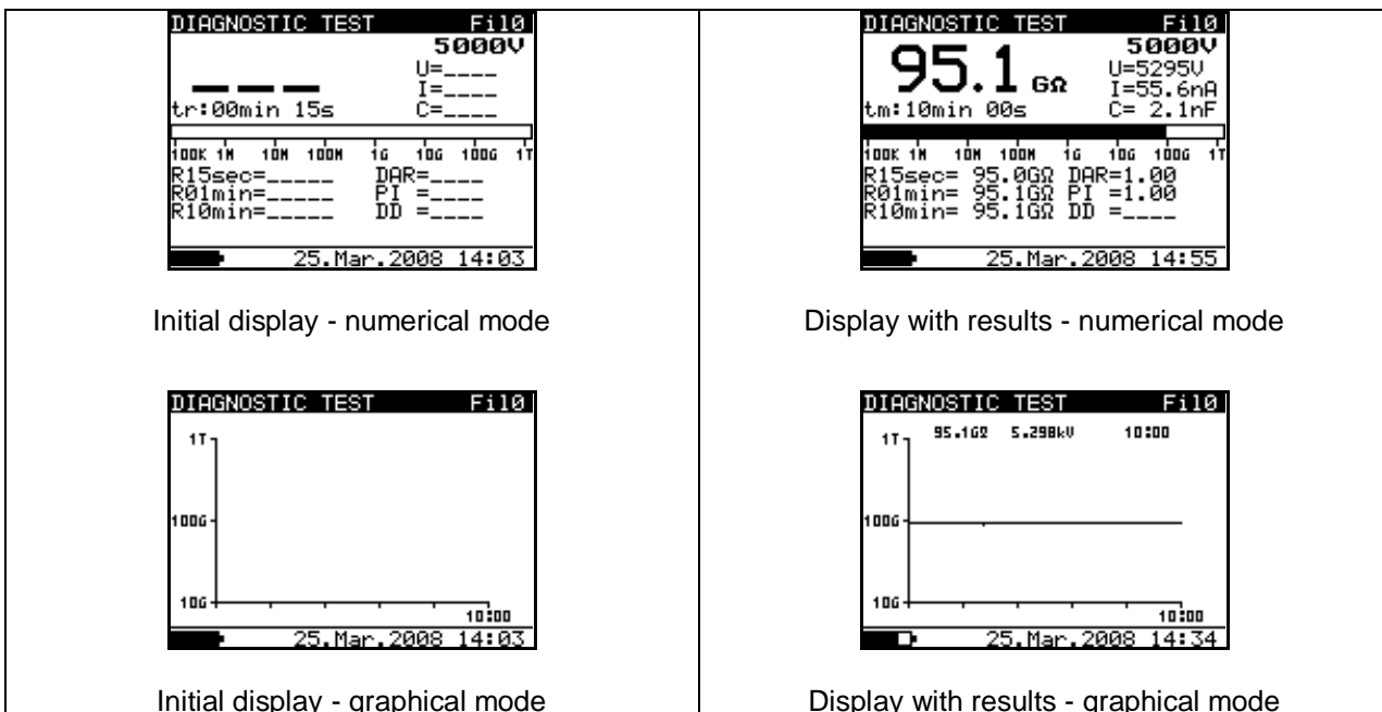
Fig. 16. Diagnostic test display states - Graph R(t) enabled
