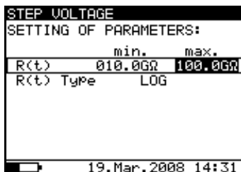
Fig. 26. Set-up menu of the Graph R(t)
