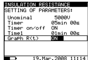
Fig. 13. Set-up menu in Insulation Resistance measurement
