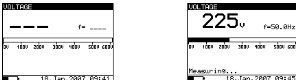
Fig. 9. Voltage function display states
