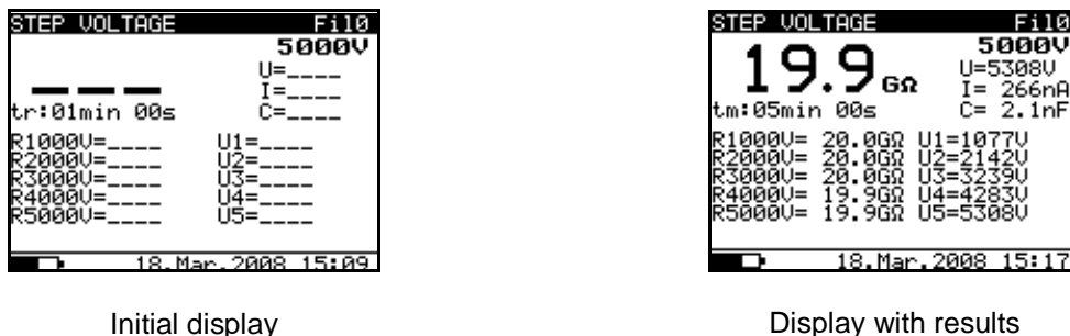
Fig. 21. Step Voltage function display states - Graph R(t) enabled
