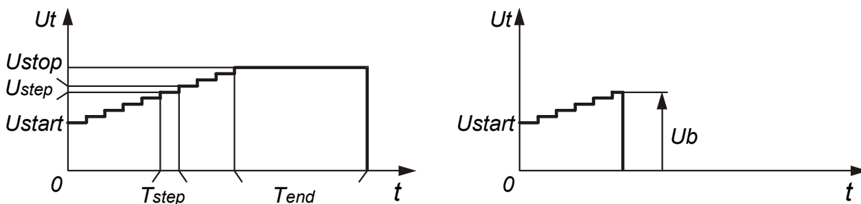
Fig. 27. Test voltage presentation without breakdown (left part) and with breakdown (right part)
