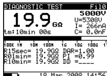
Display with results – numerical mode
