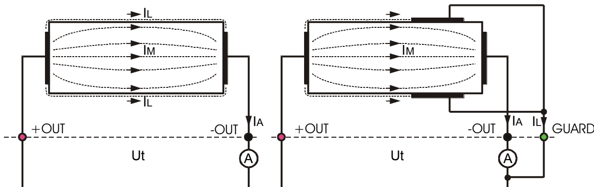
Fig. 8. Connection of GUARD terminal to measured object
