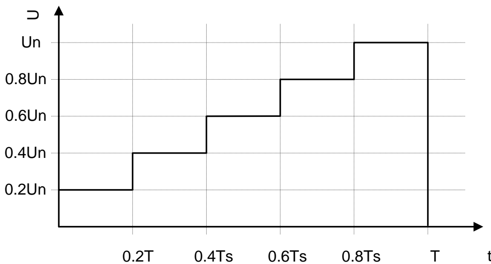
Figure 5.20 Step-up voltage test
