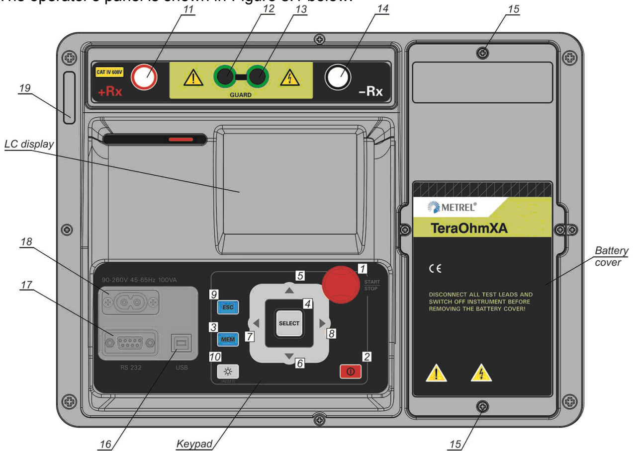
Figure 3.1: The operator’s panel
