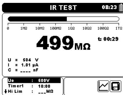
Figure 5.9: Example of Insulation resistance measurement result
