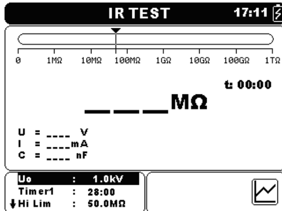
Figure 5.8: Insulation Resistance Measurement menu
