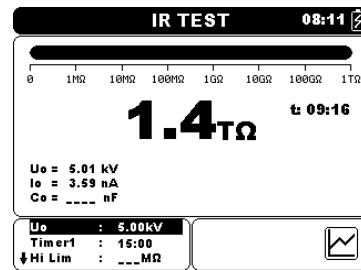
Figure 4.7: Recalled result screen
