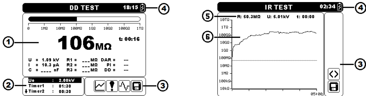
Figure 3.5: Typical function display and graph screen
